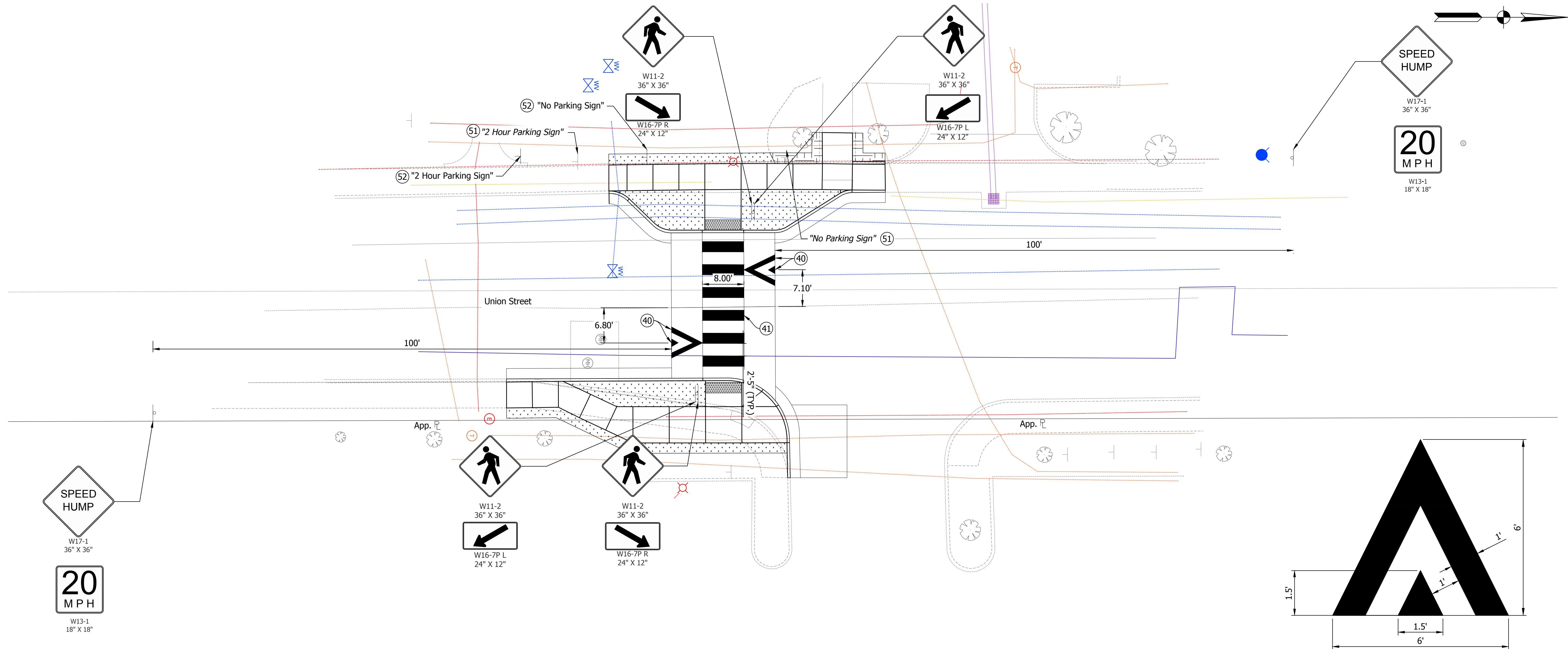
RAISED CROSSWALK MARKING DETAIL
