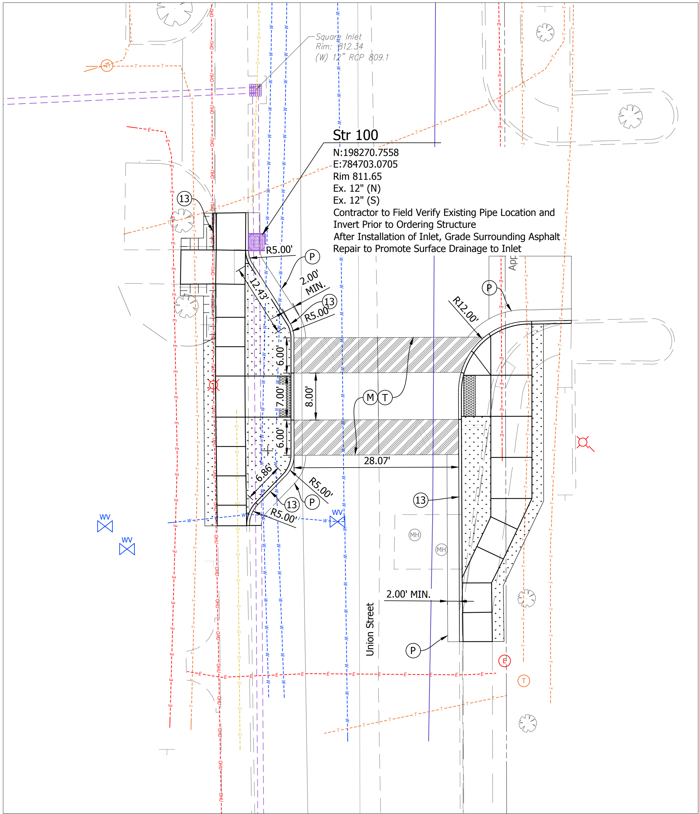
UNION STREET MID-BLOCK CROSSING
