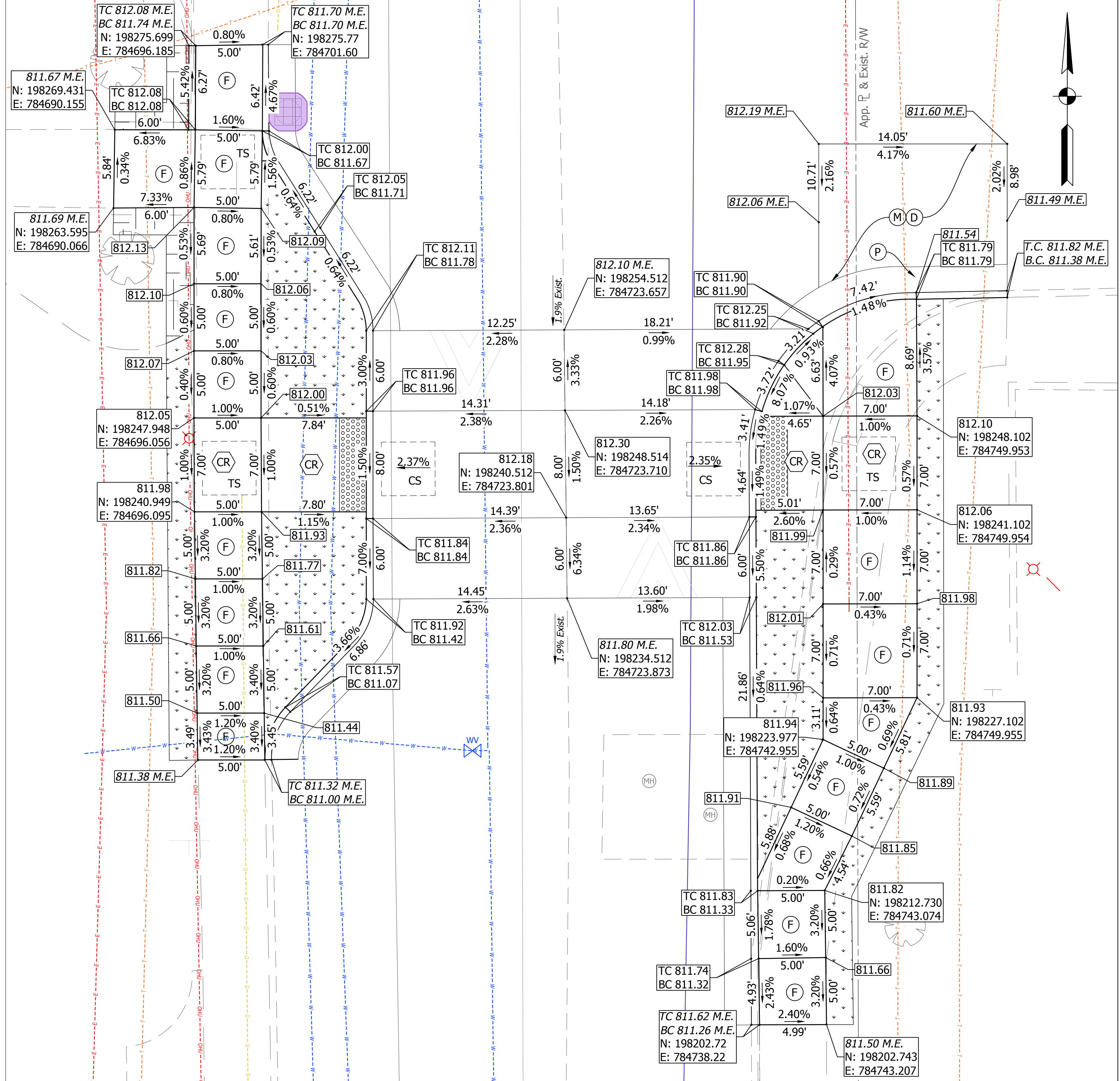
UNION STREET MID-BLOCK CROSSING CURB RAMP AND RAISED CROSSWALK DETAIL
